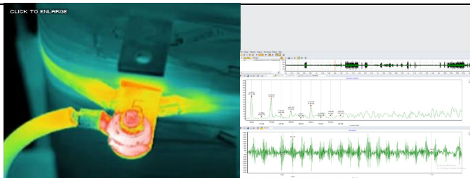
Thermal image shows hot transformer tap due to loose cable connection (Image courtesy of the Infrasppection Institute)
