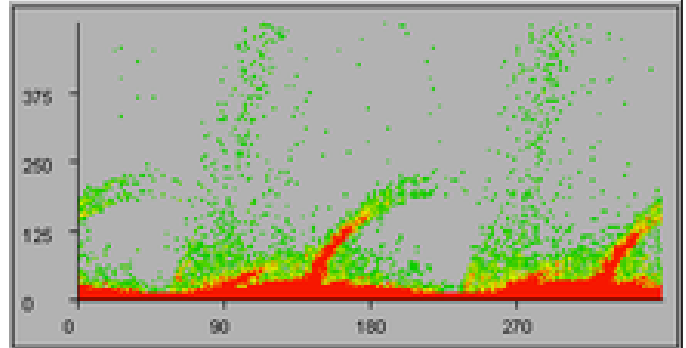
Phase-resolved partial discharge plot and surface tracking on insulator (Courtesy IPEC Ltd.)
