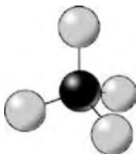
Figure 7. Methane 5 atoms per molecule
