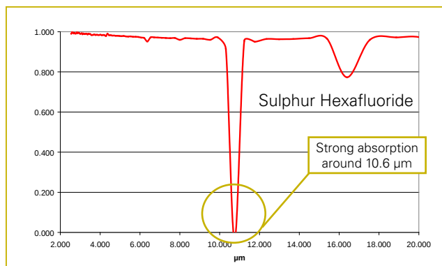
Figure 11. Sulphur Hexafluoride SF_6 – absorbent in the LW region.
