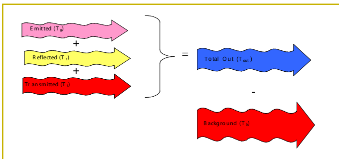
Figure 13. Radiant Contrast Of Cloud
