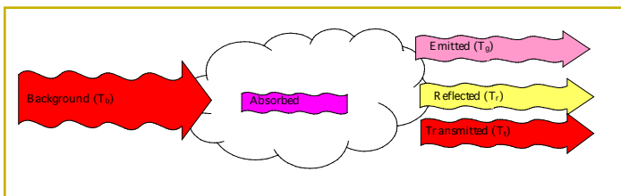
Figure 12. Effect Of A Gas Cloud
