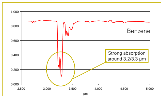
Figure 10. Benzene C_6H_6 – absorbent in the MW region
